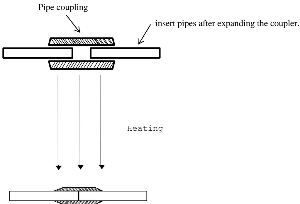
Figure 2.10: Shape Memory Alloy Pipe Coupling
