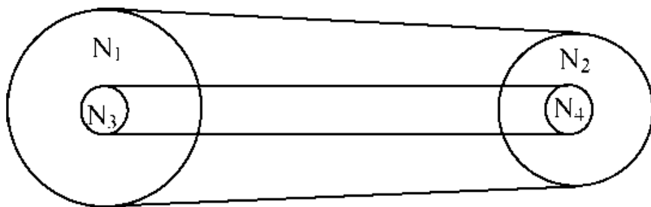
Figure 5.9: Sketch showing four sprockets with teeth numbers N_1, N_2, N_3, and N_4 .
