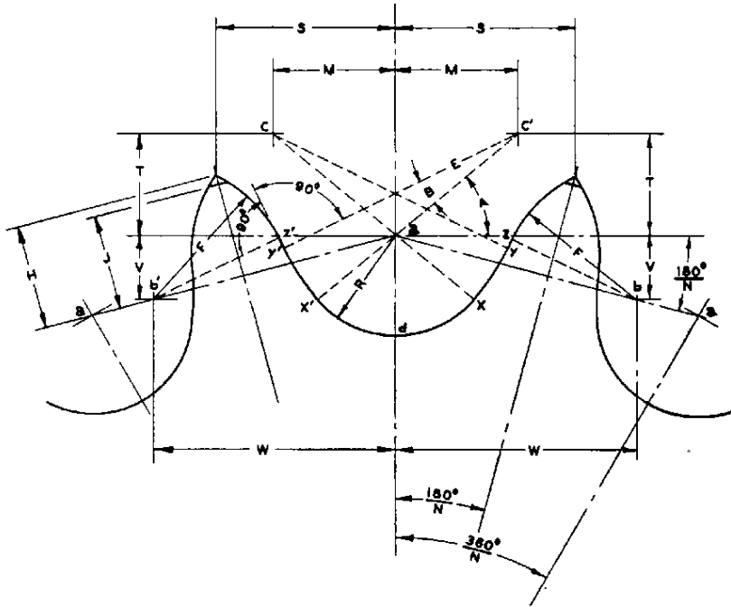
Figure 4.5: Standard sprocket tooth form for roller chains.
