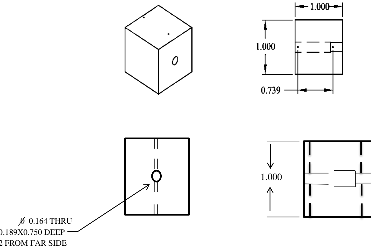
Figure 4.3: AutoCAD drawing of the fixture that holds the aluminum screw in place during machining
