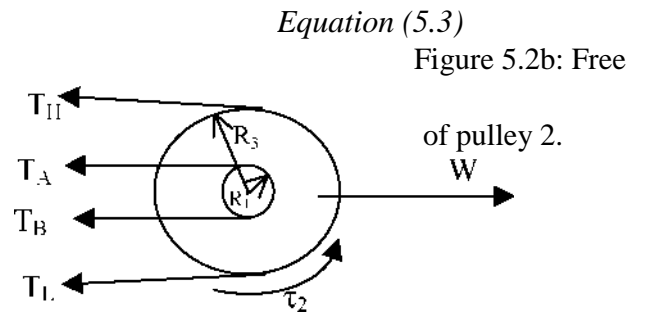
Figure 5.2b: Free body diagram of pulley 2.
