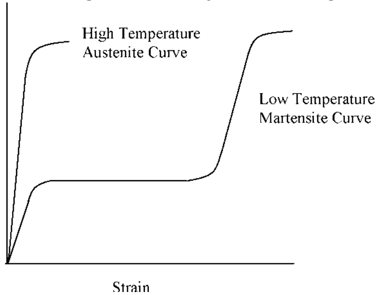
Figure 2.9: Stress-Strain Plot for comparison of the Austenite and Martensite level of stress.
