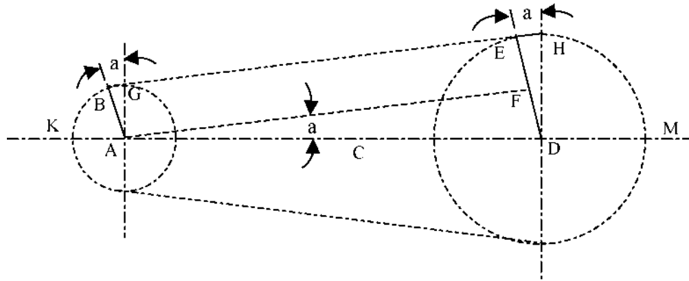
Figure 4.4: Sketch for computation of chain length
