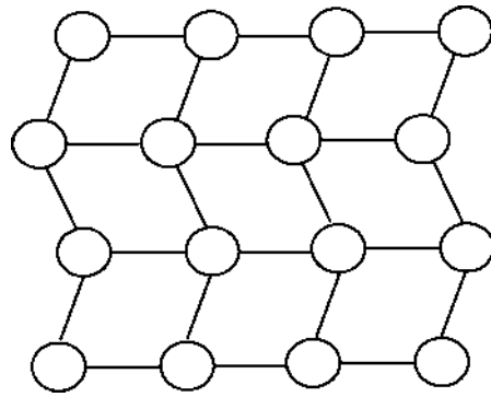
(b) : Low temperature martensite (twinned) lattice structure
