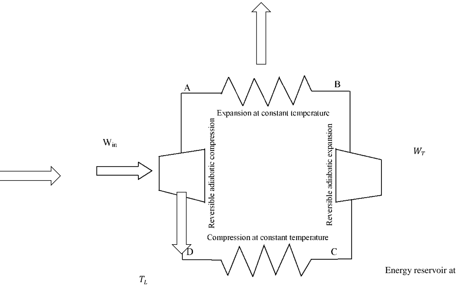
Figure 6.1: Steady-flow Carnot engine using a liquid-vapor mixture as working substance [Jones, 295]
