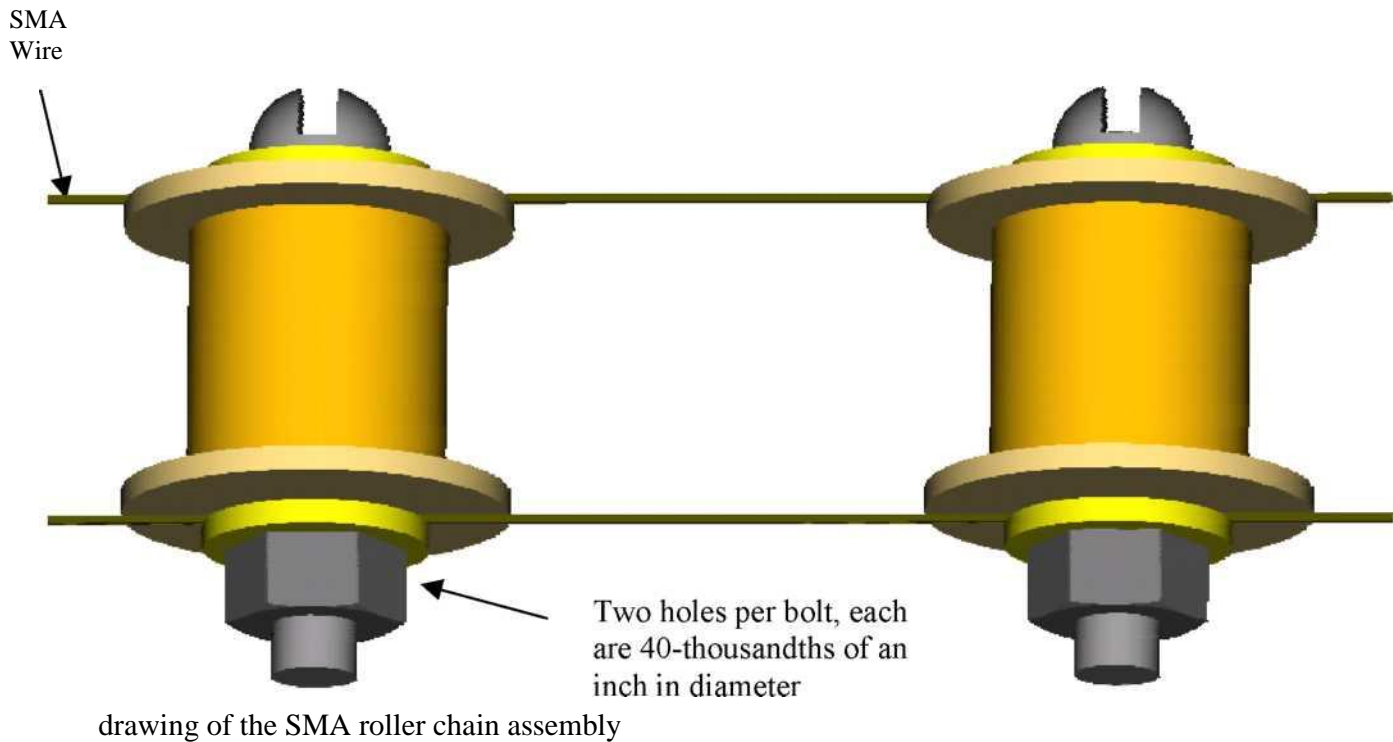
Figure 4.2: 3D CAD
