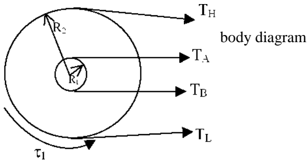
Figure 5.2a: Free body diagram of pulley 1.
