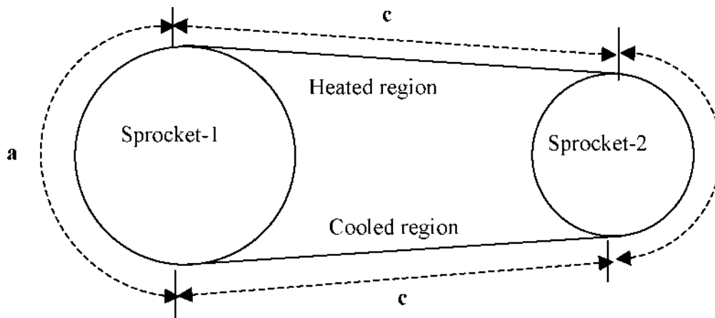
Figure 5.4: Sprocket-1 sweeps more material than sprocket-2, stretching the chain in the cooled region and damping more material in heated region.
