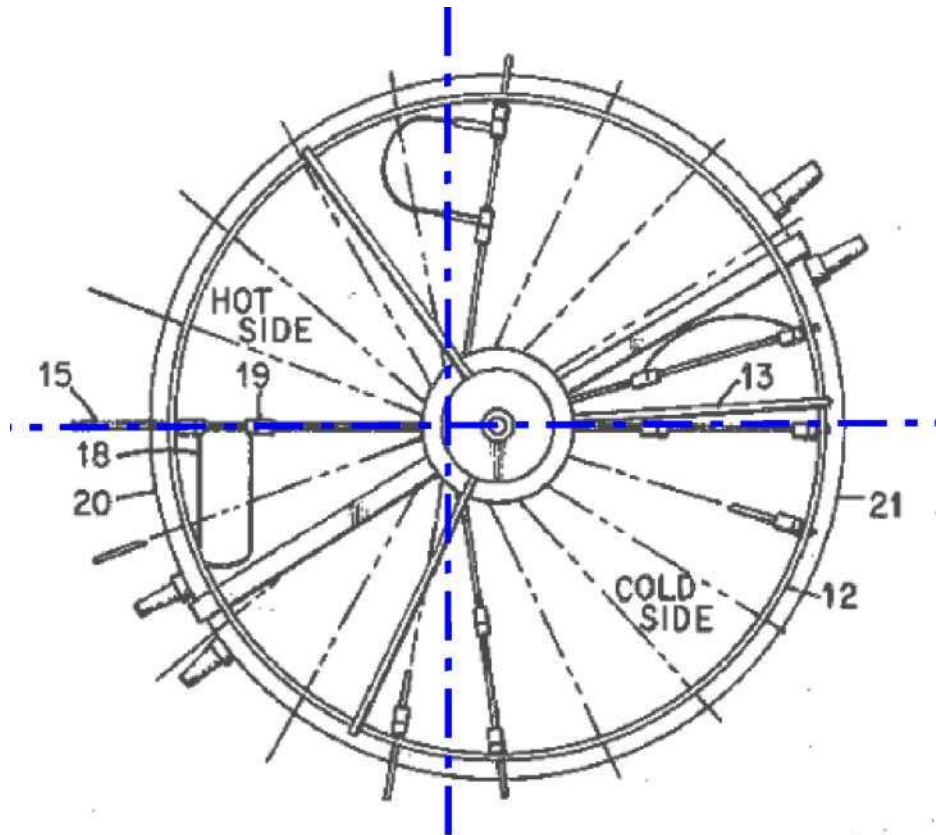
Figure 3.2: A plan view of Banks' heat engine
