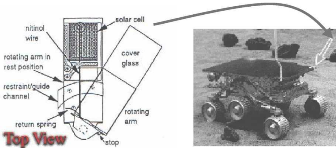
Figure 2.14: The Mars Pathfinder used a Nitinol actuation for the first time outside the earth's atmosphere
