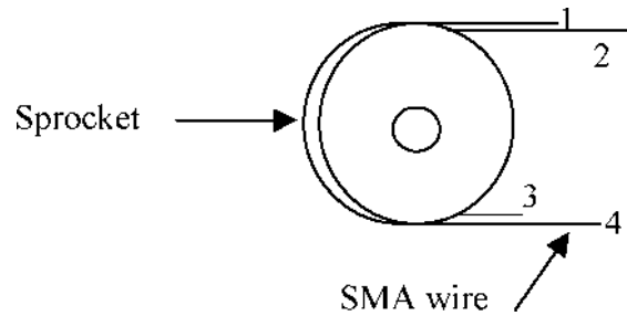
Figure 4.7: Sketch of sprocket showing the four wires that are part of the SMA chain
